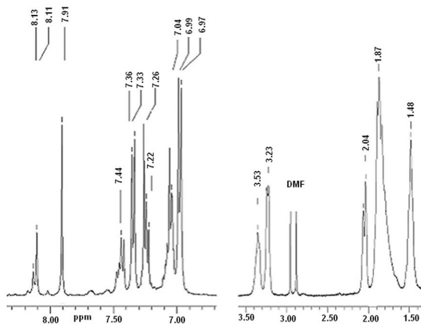
Fig. 3 ^1\text{H} -NMR spectrum ( \text{CDCl}_3 , 25 °C) of 3a , (presented in Fig. 2) registered again after several days.
